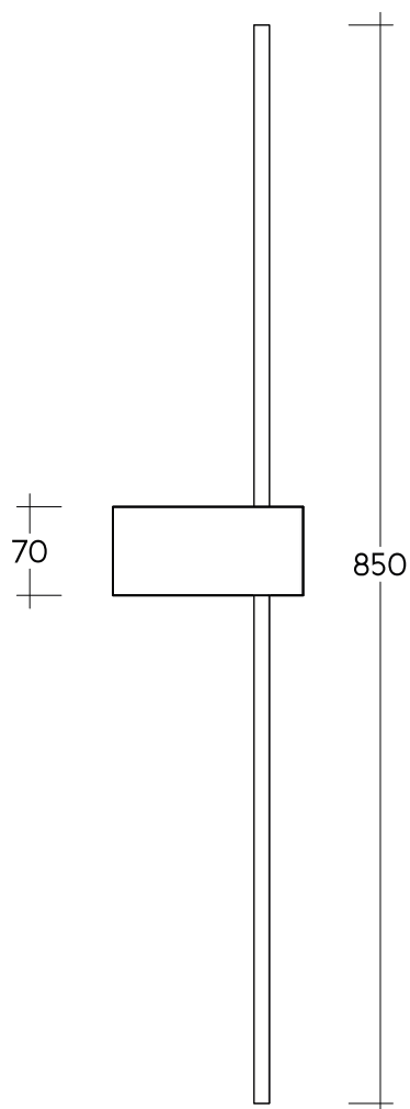
ΟΨΗ . ELEVATION
